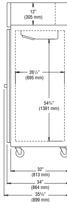
RIGHT VIEW
